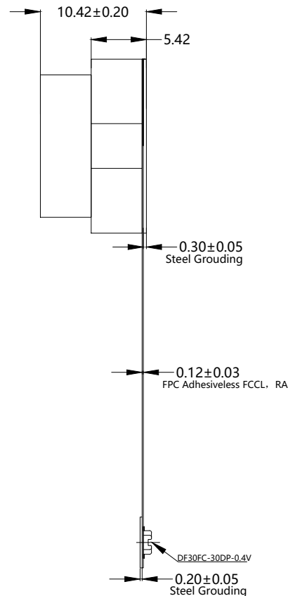
SIDE VIEW
